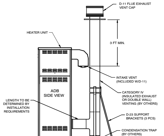
OUTDOOR TERMINATION STACK
