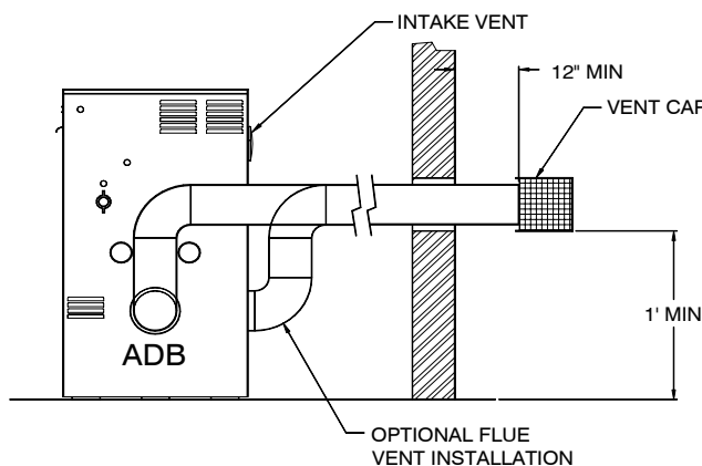
SIDEWALL TERMINATION
