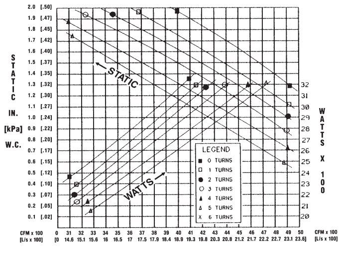
10 TON [35 kW] O DRIVE (3Ø only)
