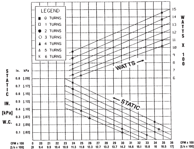
10 TON [35 kW] (RHGG-120 ONLY) J DRIVE (3Ø only)
