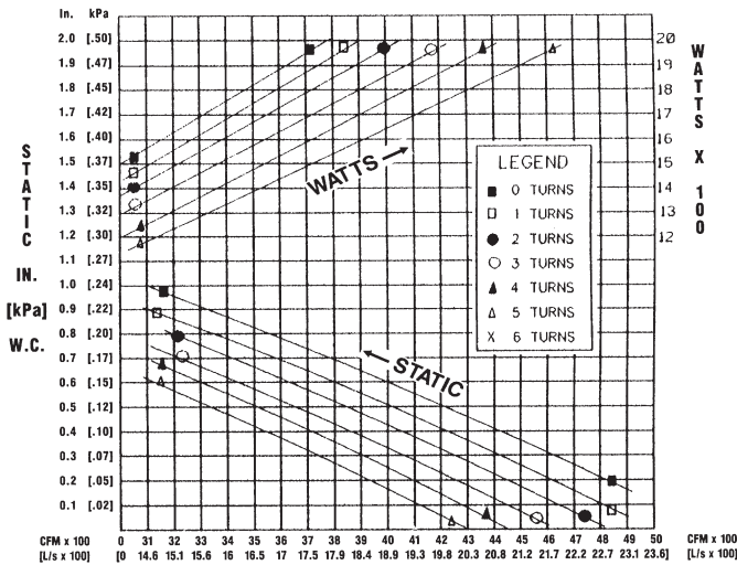
10 TON [35 kW] L DRIVE (3Ø only)
