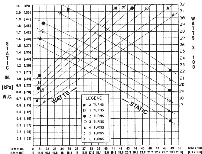
10 TON [35 kW] N DRIVE (3Ø only)
