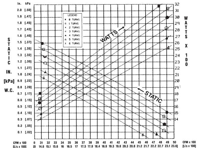
10 TON [35 kW] M DRIVE (3Ø only)
