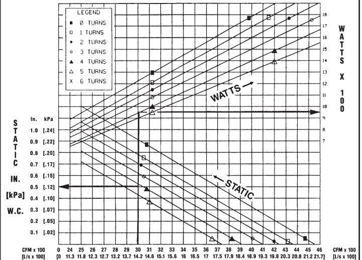
10 TON [35 kW] K DRIVE (3Ø only)
