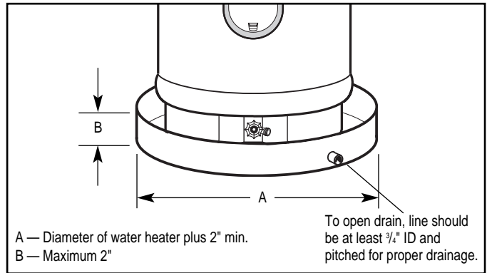
Figure 1. — Auxiliary Drain Pan
