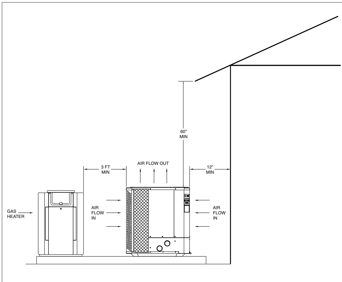
Fig. 1: Installation Clearances
