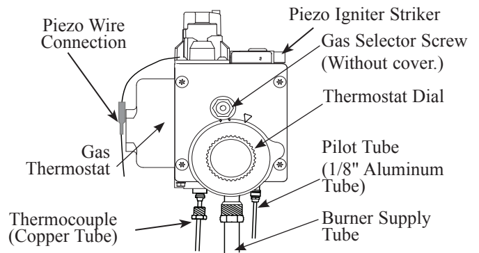
Front View of Gas Thermostat
