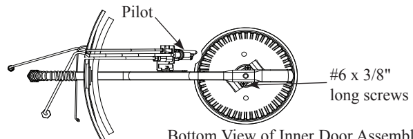
Bottom View of Inner Door Assembly
