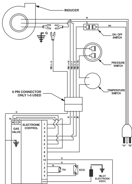
Connection Diagram
