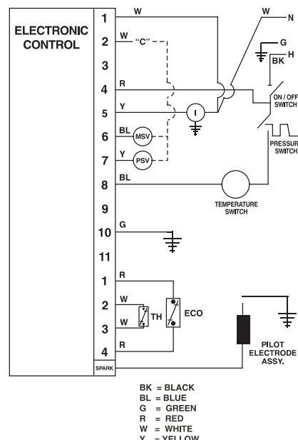
Schematic Diagram
