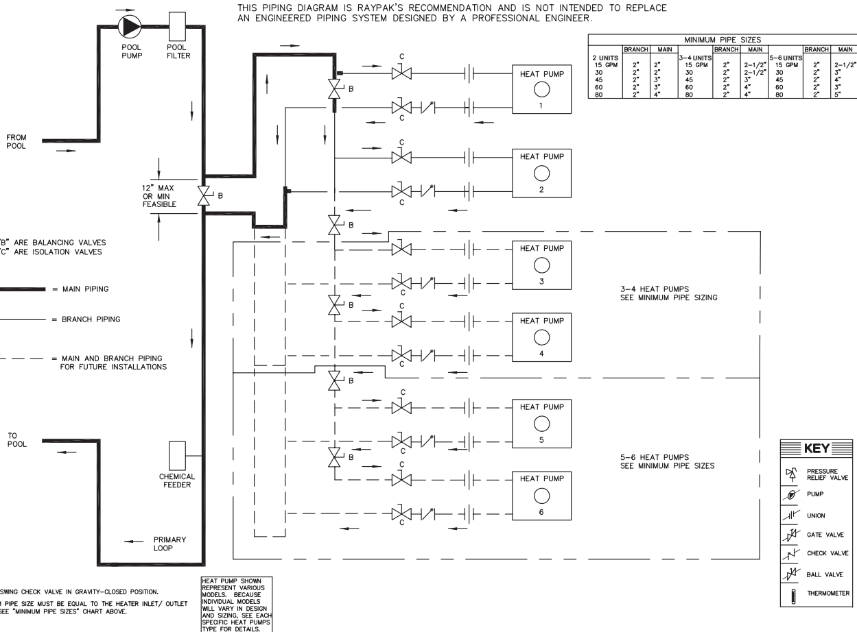
Fig. 9: Pool Piping for Heat Pump Pool Heaters, Multiple, Primary/Secondary
