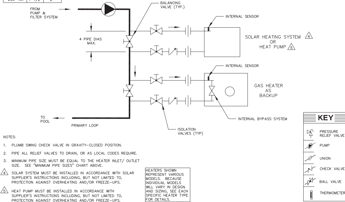
Fig. 8: Pool Piping for Heat Pump Pool Heater and Gas Pool Heater
