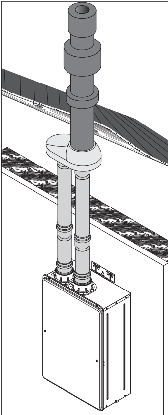
ICRT2439 Concentric Roof Termination
